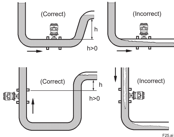
Mounting Positions
